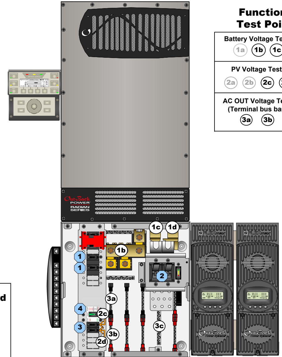
Test points 2c and 2d refer to the right terminal of each circuit breaker.
