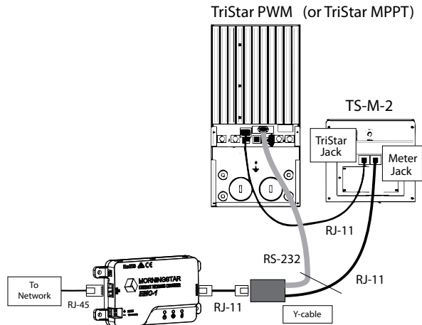
Figure 2-2. EMC-TS-M-2 Cable Routing
