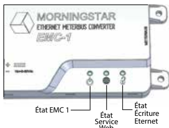
Figure 3-1. Voyants DEL
