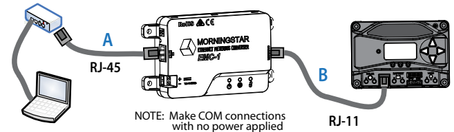
Figure 2-1. Connecting the COM cables
